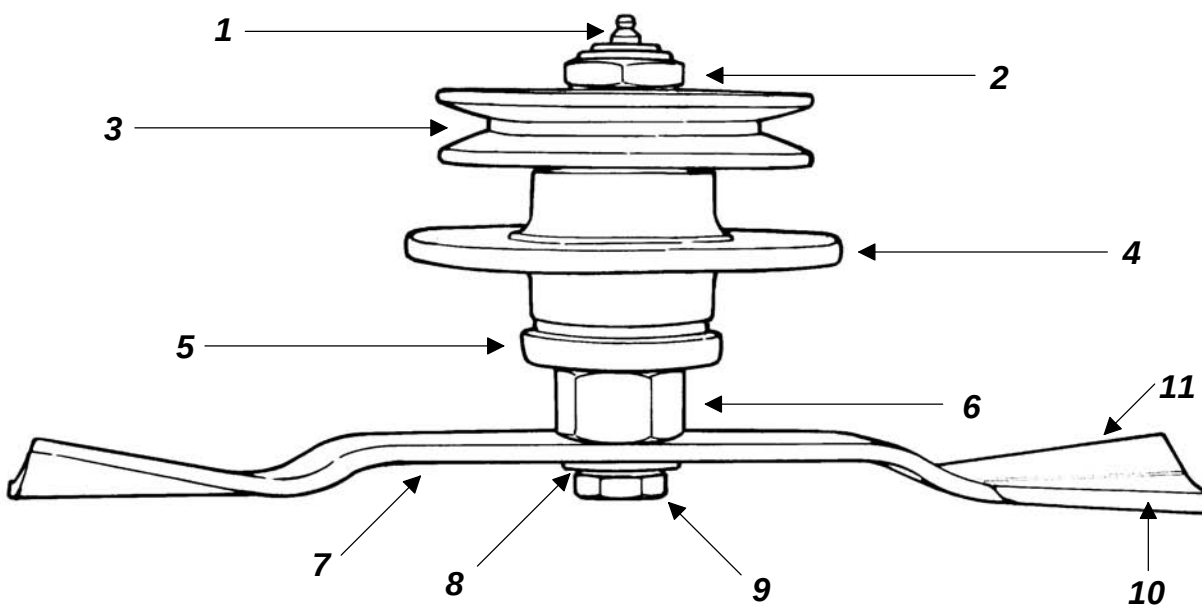
Fig. 7 - Spindle assembly.
